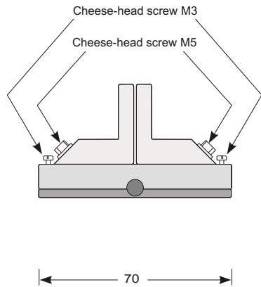
Base part 1.0 FIG. 1.1
