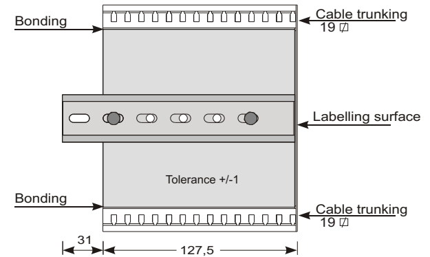
Mounting part M 125 (ES/DS)
