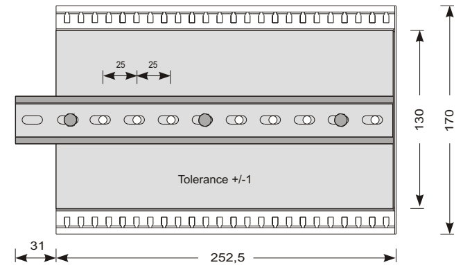
Mounting part M 250 (ES/DS) FIG. 2
